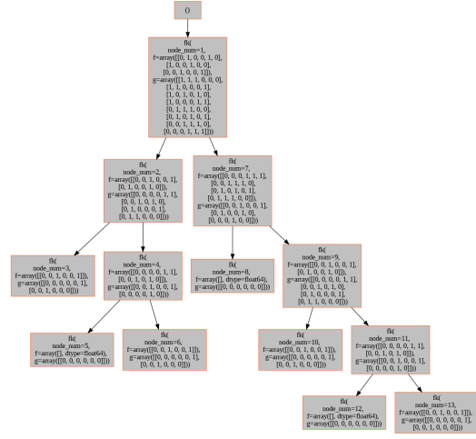
(b) Visualization of 6-B in FK-A
