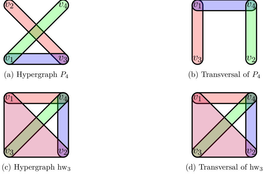
Figure 3.5: Hypergraph P_4 and its transversal. Hypergraph hw_3 and its transversal.
