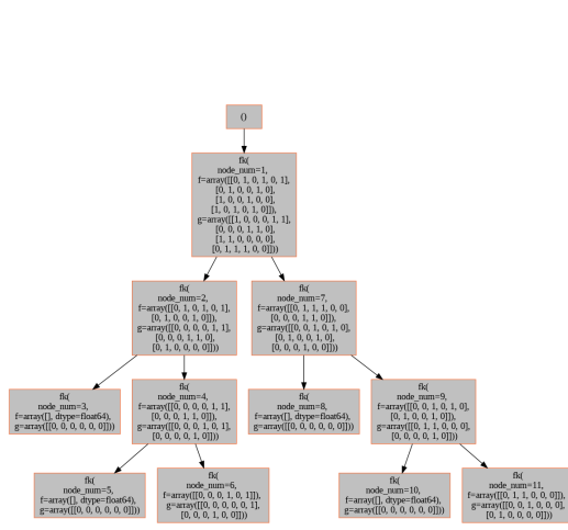
(a) Visualization of 6-A in FK-A
