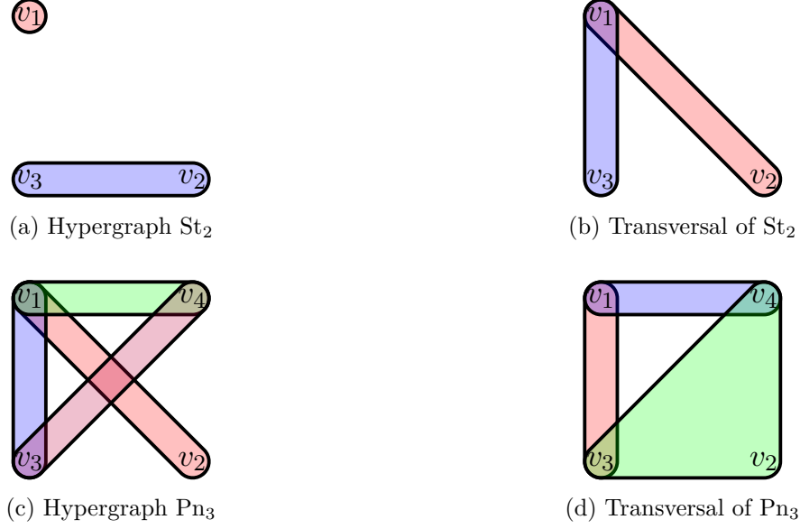
Figure 3.1: Hypergraphs St_2 and Pn_3 and their transversals.
