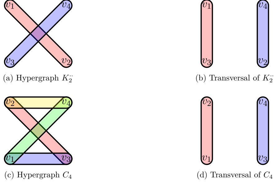
Figure 3.6: Hypergraph K_2 and its transversal. Hypergraph C_4 and its transversal.
