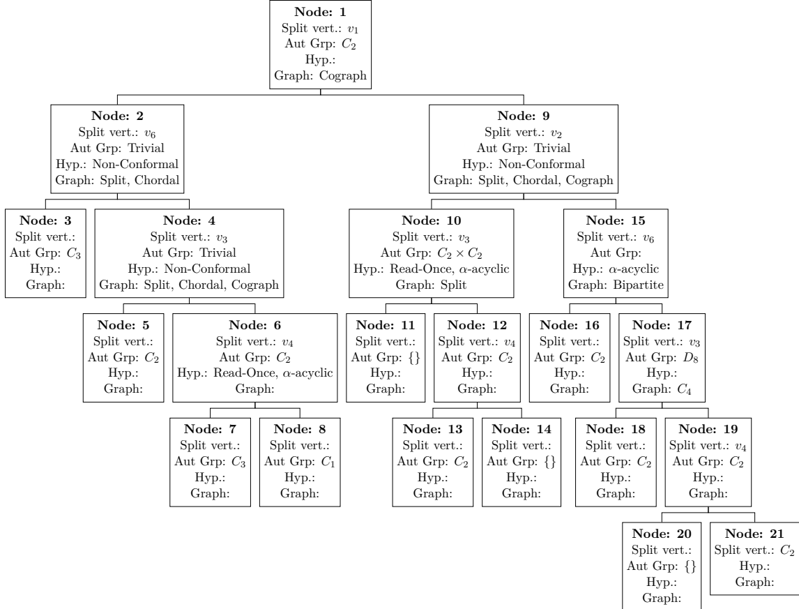
(b) Automorphism Tree of 7-ver Hypergraph in FK-A
