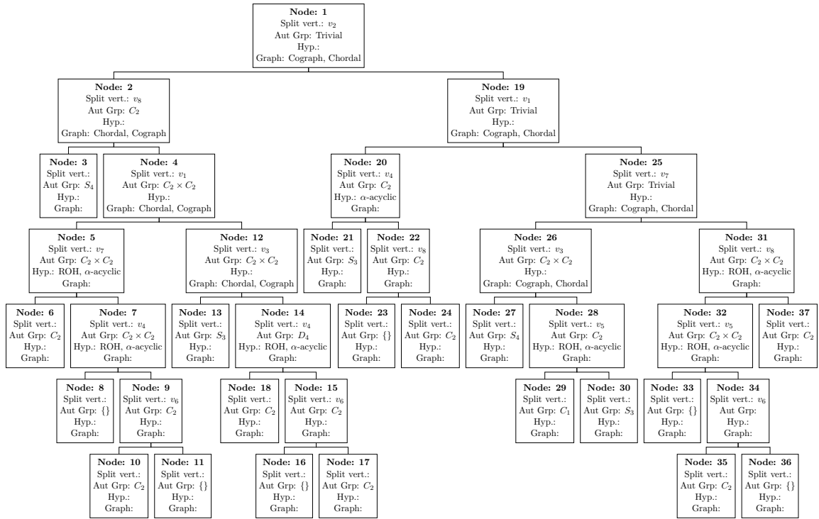
Figure 8: Automorphism Tree of an asymmetric hypergraph Asym-1 in FK-A
