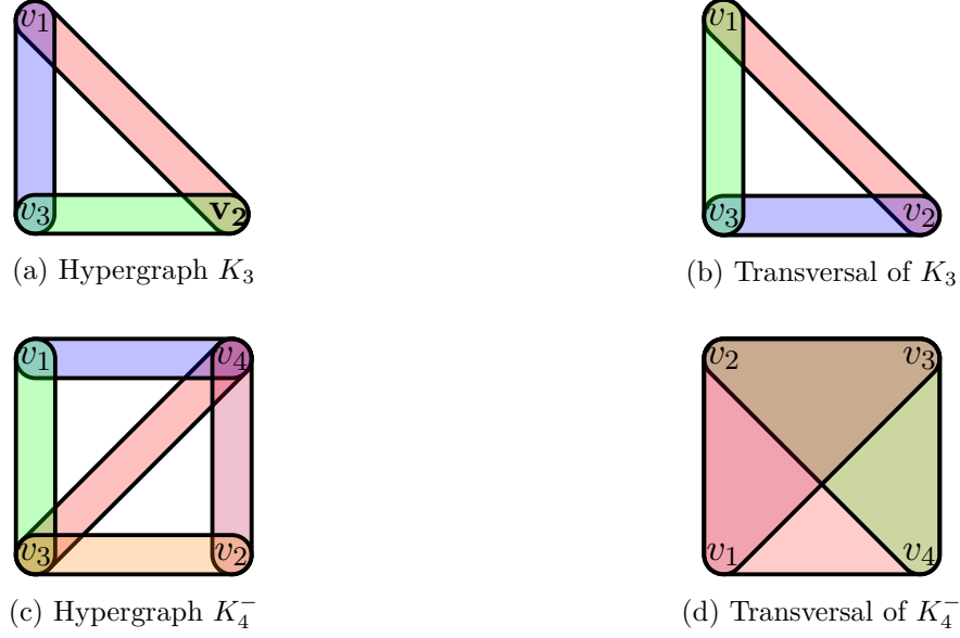
Figure 3.4: Hypergraph K_3 and its transversal. Hypergraph K_4^- and its transversal.
