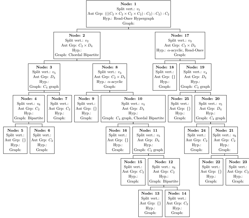
(a) Automorphism Tree of f_2, g_2 from \mathcal{GK} -family in FK-A
