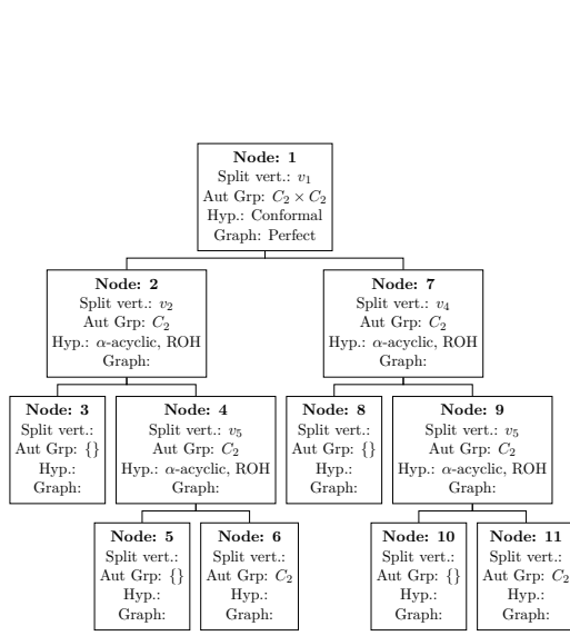
(a) Automorphism Tree of Hypergraph 6A from [SS24] in FK-A.
