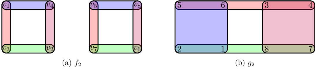
Figure 4.1: Hypergraphs f_2 and g_2 in the \mathcal{GK} -family.
