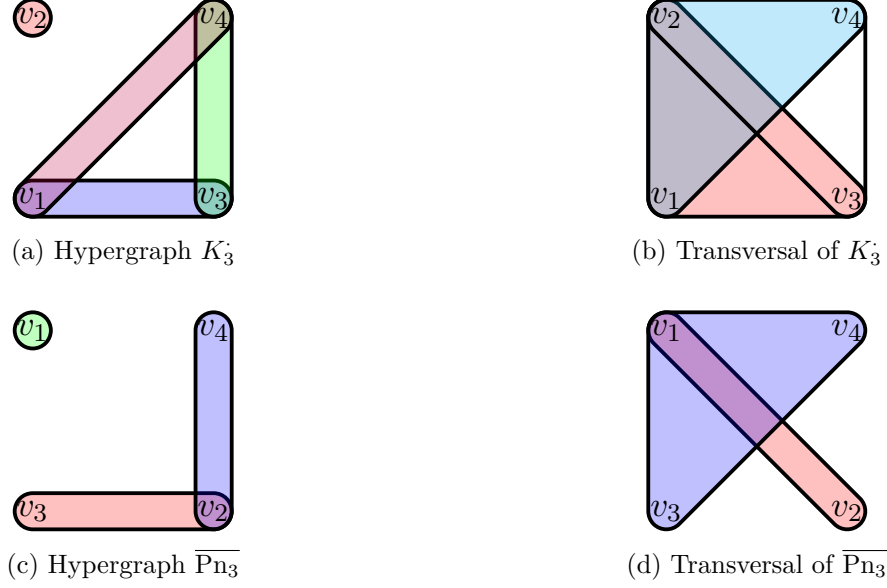
Figure 3.2: Hypergraph K_3 and its transversal. Hypergraph \overline{Pn_3} and its transversal.
