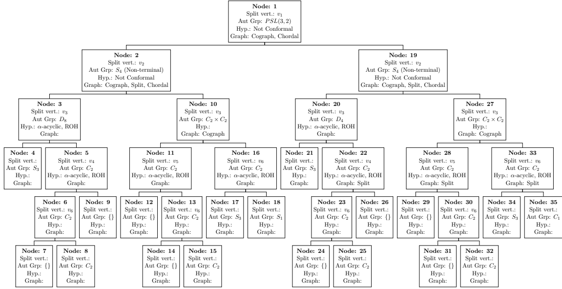
(a) Automorphism Tree of Self-Transversal Fano Plane Hypergraph in FK-A
