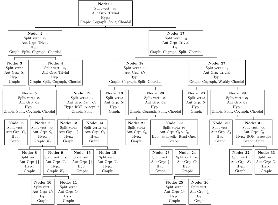
Figure 10: Automorphism Tree of an asymmetric hypergraph Asym-2in FK-A
