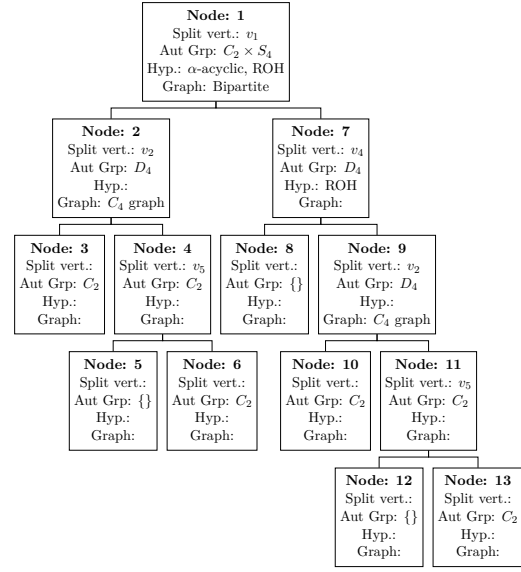
(b) Automorphism Tree of ROH Hypergraph 6B from [SS24] in FK-A.
