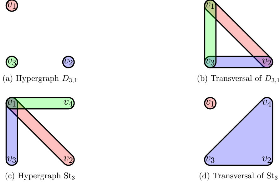
Figure 3.3: Hypergraph D_{3,1} and its transversal. Hypergraph St_3 and its transversal.
