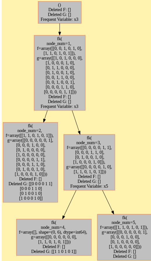
(c) Visualization of 6-C in FK-A
