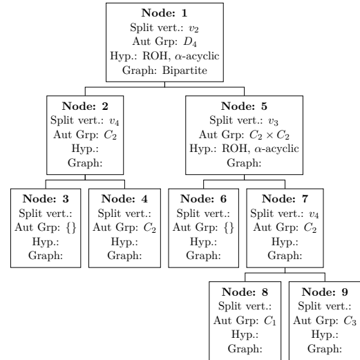
(d) Automorphism Tree of Hypergraph 6D from [SS24] in FK-A.
