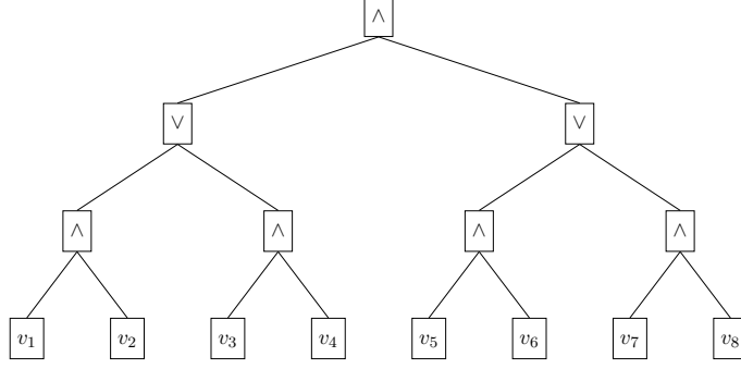
Figure 4.2: Alternating Tree g_2 in \mathcal{GK} family
