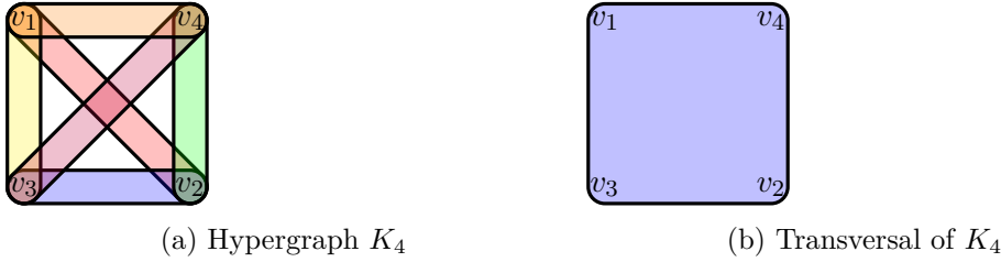
Figure 3.7: Hypergraph K_4 and its transversal.
