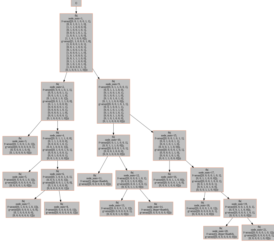
(a) Visualization of 7-vertex Hypergraph in FK-A
